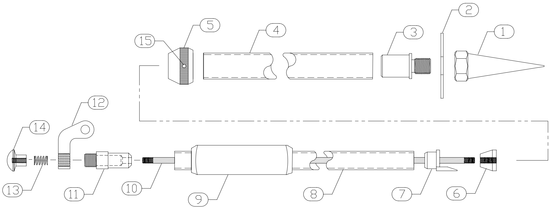
Bipod/Tripod Leg Assy.
